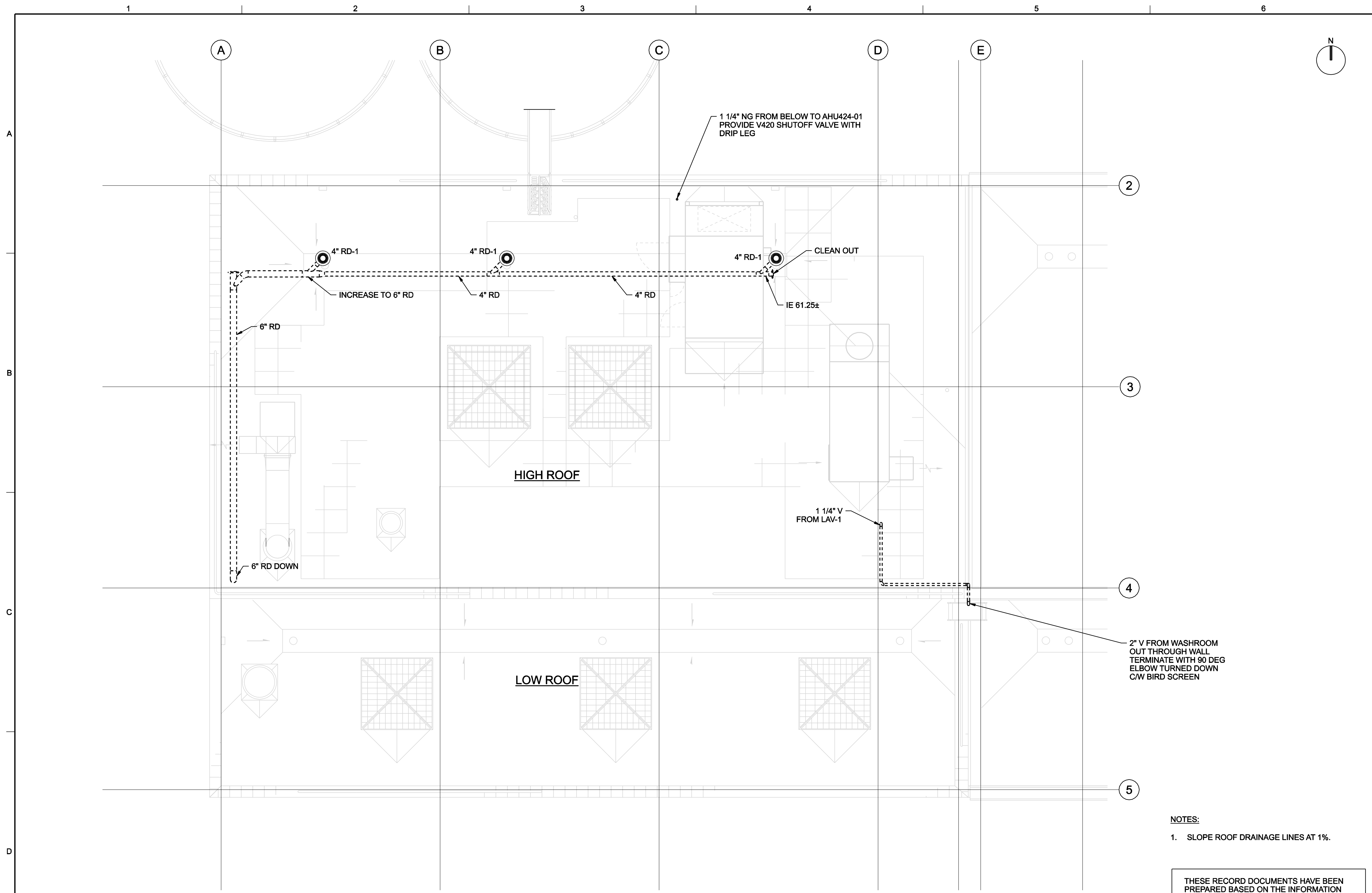
1 ROOF PLAN 1/4"=1'-0"
