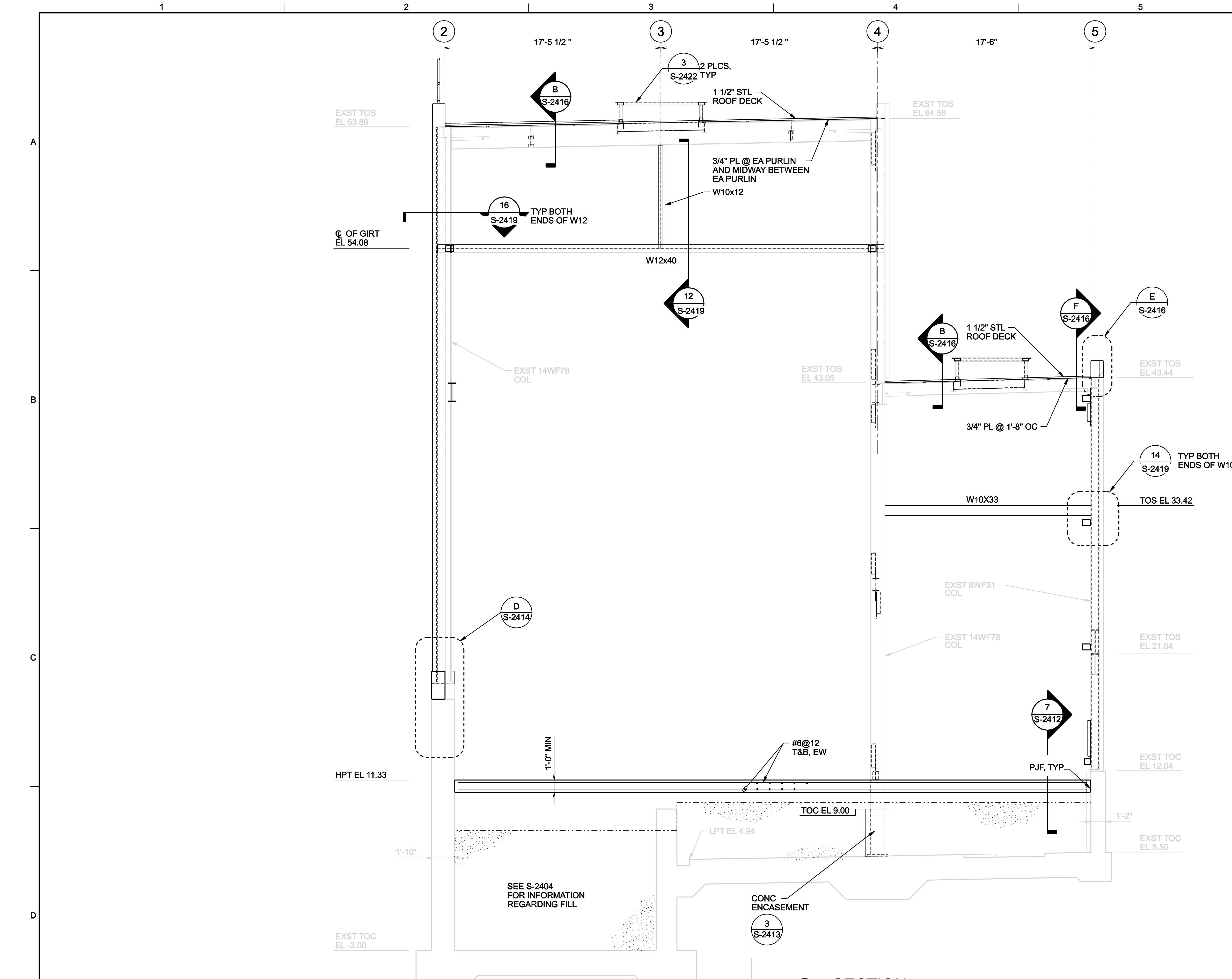
C SECTION 1/4"=1'-0" S-2400, S-2401 S-2402
