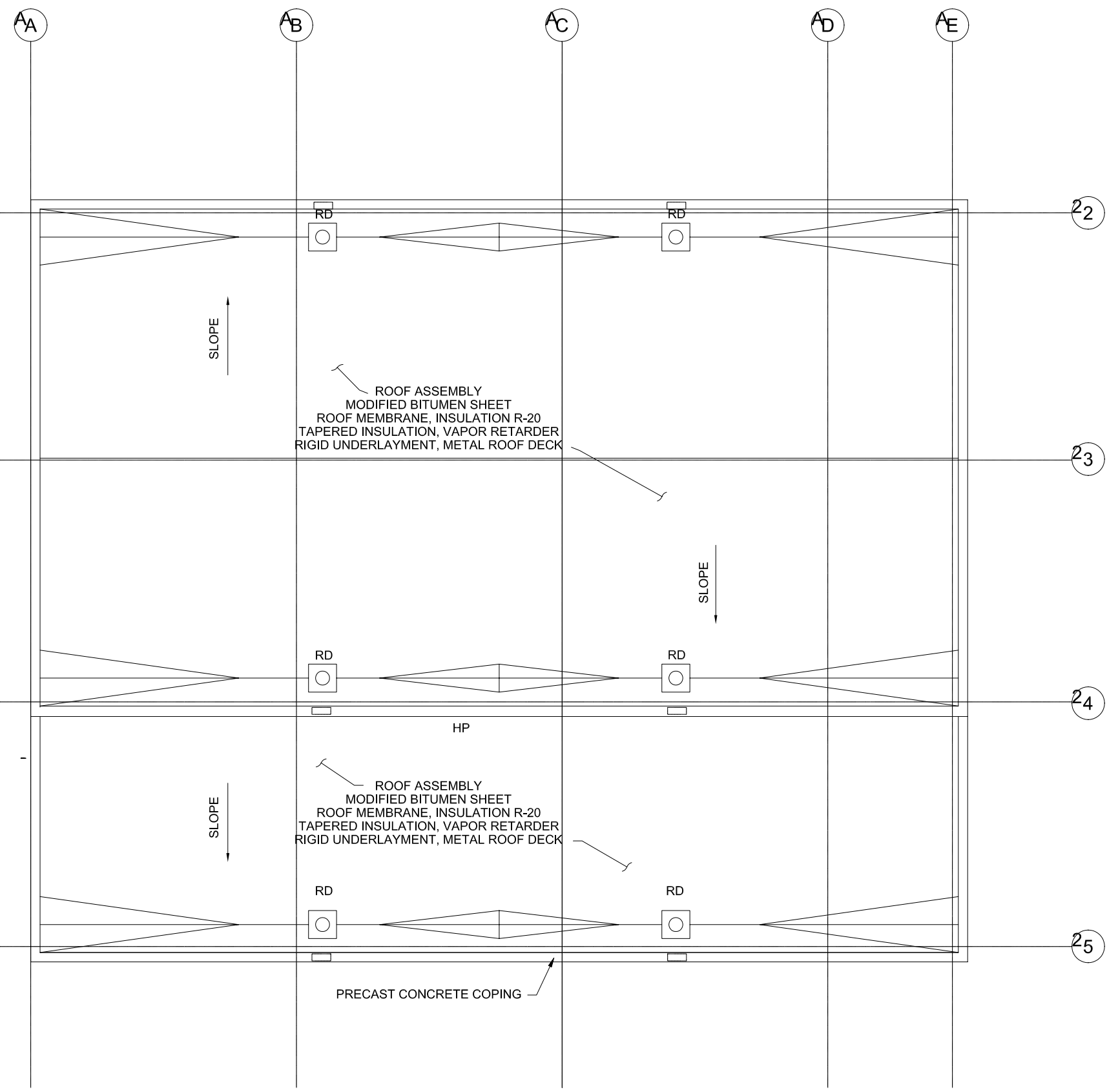
ARCHITECTURAL ROOF PLAN
