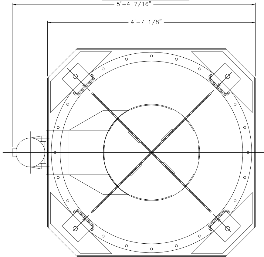
ELEVATION VIEW 5'-4 7/16"
