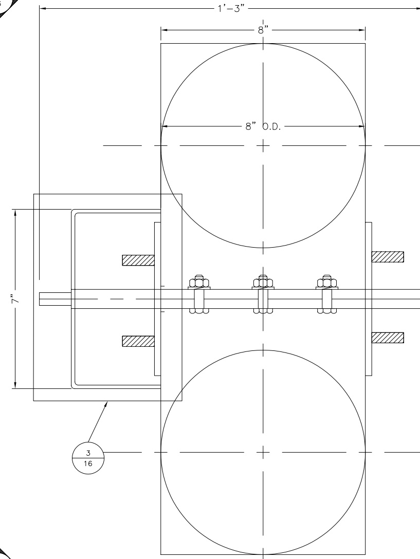
A VIEW 6"=1'-0"
