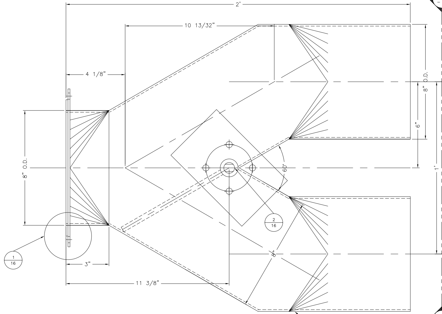
PLAN VIEW
