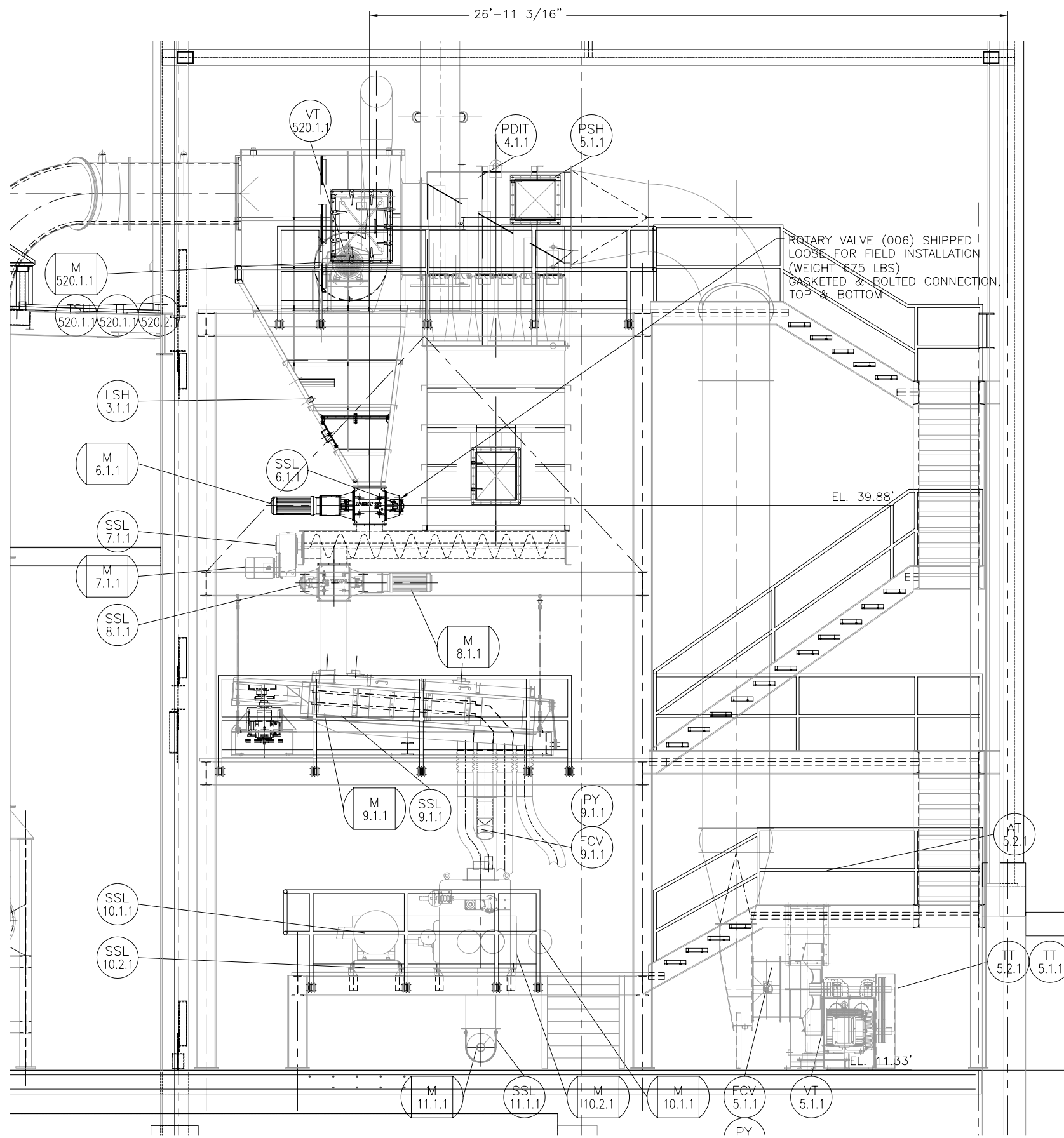
ELEVATION VIEW
